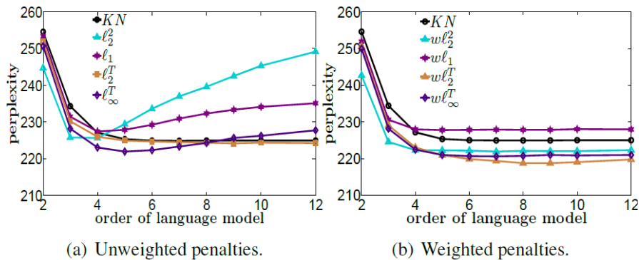
Figure 6. The classical measure of performance for natural language models is the perplexity (lower is better). Our models are denoted by \ell_2^T and \ell_\infty^T .
